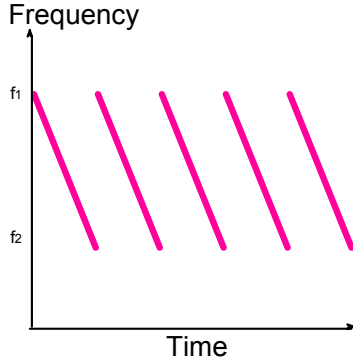
Fig. 2 Frequency modulation for a CPA.
