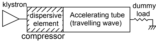
Fig. 3 Schematic layout for a RF-CPA.
