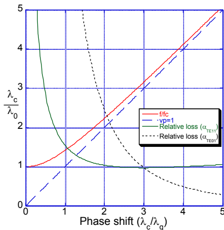
Fig. 4 Brillouin diagram of a plain wave guide.
