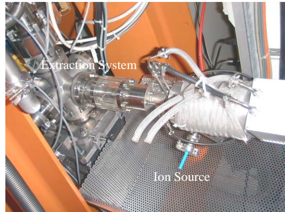
Figure 5: The REX test ion source mounted on the separator magnet. The plasma chamber and the extraction electrode is inside the transparent flange. The rectangular box on the right hand side houses the magnetron.
