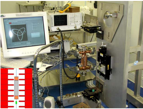
Fig.5. The general arrangement of the bead-pull set-up.
