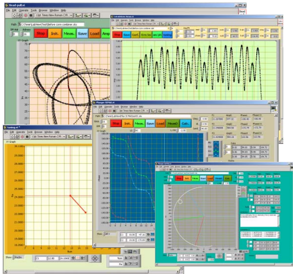
Fig.6. The windows of LabView program for bead-pull measurements and complete structure tuning
