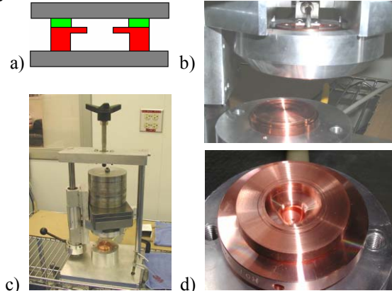
Fig.1. a) Schematic view. b) Bottom block and upper floating block. c) General view of set-up. d) Cup and half-cell installed on bottom block.
