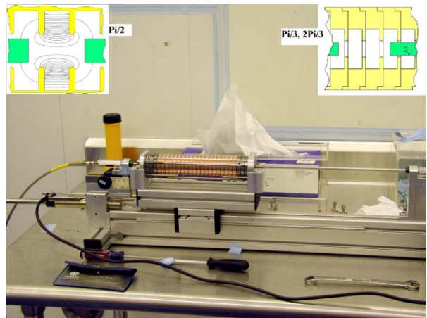
Fig.3. The plunger set-up.
