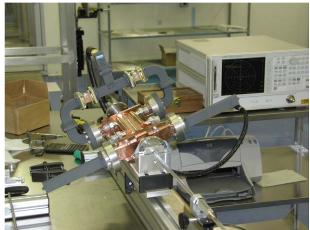
Fig.4. The plunger set-up for nodal measurements.
