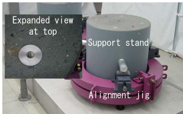
Figure 4: Full size support stand and attaching alignment jig were developed by Takenaka Co. The surface roughness and flatness are within \pm 10 \mu\text{m} .
