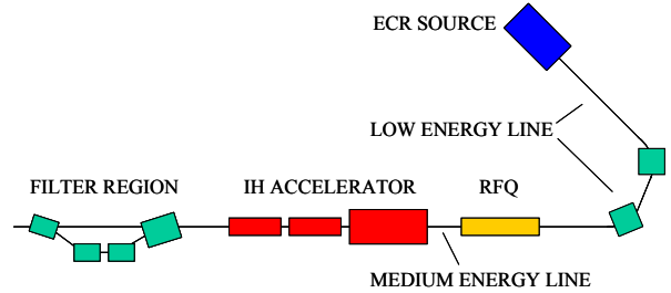
Figure 1. Layout of the present CERN Linac 3 heavy ion pre-injector.
