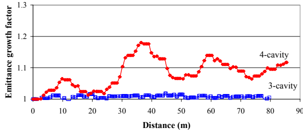
Figure 6: The 99.9% emittance-growth factor in the vertical plane along the first section of the ECL, \mu_t=90^\circ .
