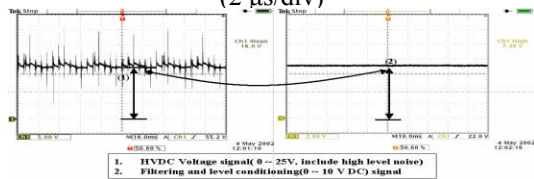
Fig. 4. Pre-conditioned waveform of HVDC voltage (10 ms/div)
