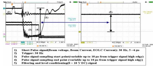
Fig. 3. Pre-conditioned waveform of short pulse signal (2 \mu s/div)
