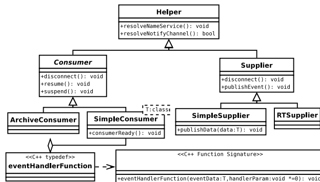
Figure 1: ACS Notification Channel API class model.
