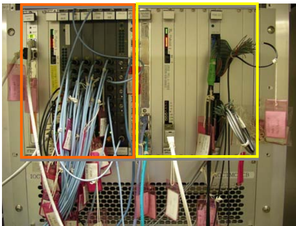
Figure 3: VME divided (Right: CPU5500)
