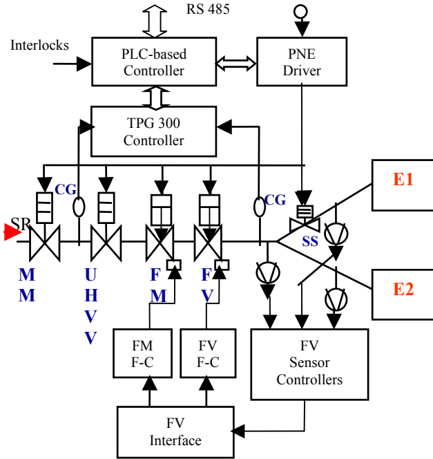
Figure 2: Schematic block diagram of a typical new PLC-based EPS system for 1W1 high-power beamlines: (SR) synchrotron radiation, fast valve (FV), fast mask (FM), movable mask (MM), UHV valve (UHV), (CG) cold cathode gauge, (FV-FC) fast valve firing circuit, (FM-FC) fast mask firing circuit, (SS) safety shutter, (PNE Driver) pneumatic driver for the valves and safety shutters, (E1, E2) experimental station 1 and 2.
