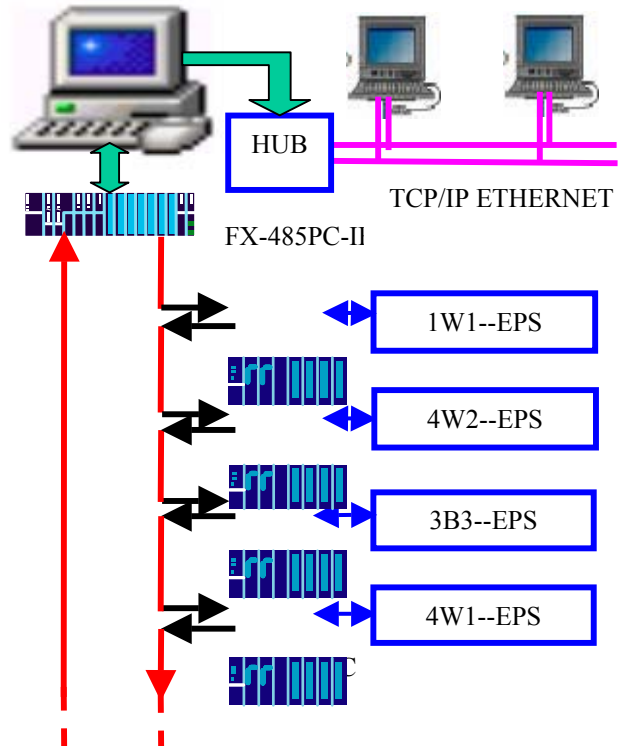
Figure 3: Block diagram of the hardware configuration for the centralized monitoring system.
