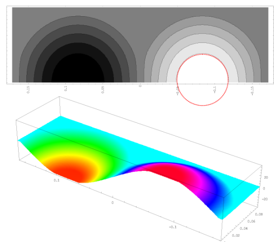
Fig. 6: Contour plot of the integrated accelerating voltage.
