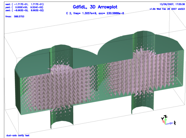
Fig. 1: A conceptual dual-axis single-cell cavity.
