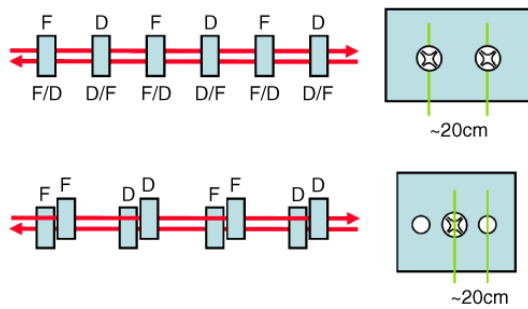
Fig. 7: Conceptual optics layout with dual-axis quadrupoles.
