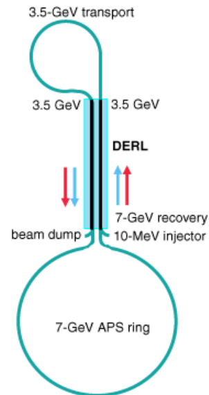
Fig. 3: DERL as a recirculating linac. It functions as two separate ERLs with no power transfer between the two axes.
