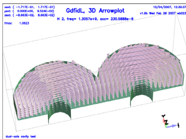
Fig. 4: Magnetic field of the accelerating eigenmode shown in Fig. 1.
