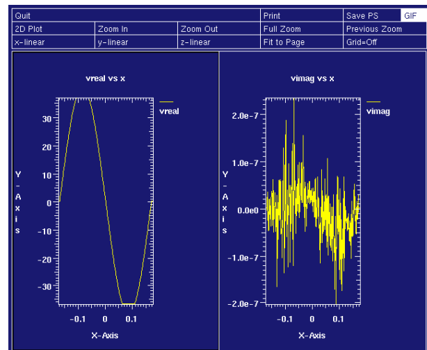
Fig. 5: Integrated accelerating voltage across the cavity. Note the flat tops within beam pipes which are desired for beam acceleration.
