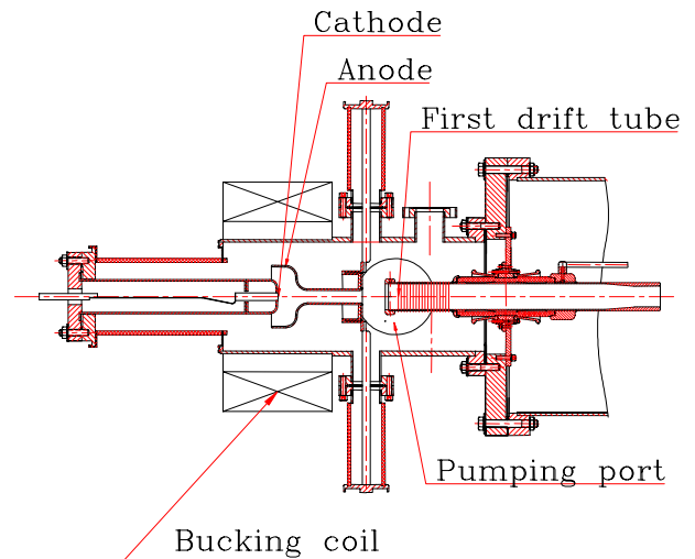
Figure 2: Schematic of the 10 A electron gun.
