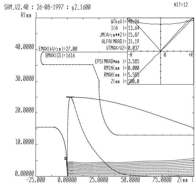
Figure 3: Electron gun optics simulation.
