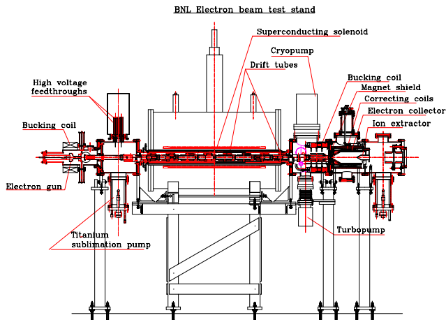
Figure 1: Layout of the electron beam test stand.
