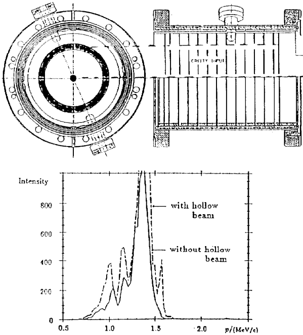
Fig. 3. The wake-field accelerator developed by the DESY group. A drive beam of 6 bunches, each of 5 nC, and separated by 2 ns, resonantly excited the structure and accelerated particles. The inferred gradient was 1.2 MeV/m over 16 cm. (Bialowons, et al 1987)
