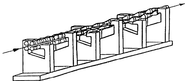
Fig. 2. Schematic drawing of a four-rod RFQ.
