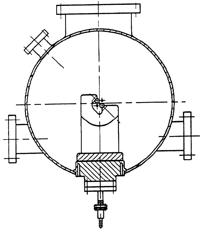
Fig. 6. Cross section of the four-rod RFQ.
