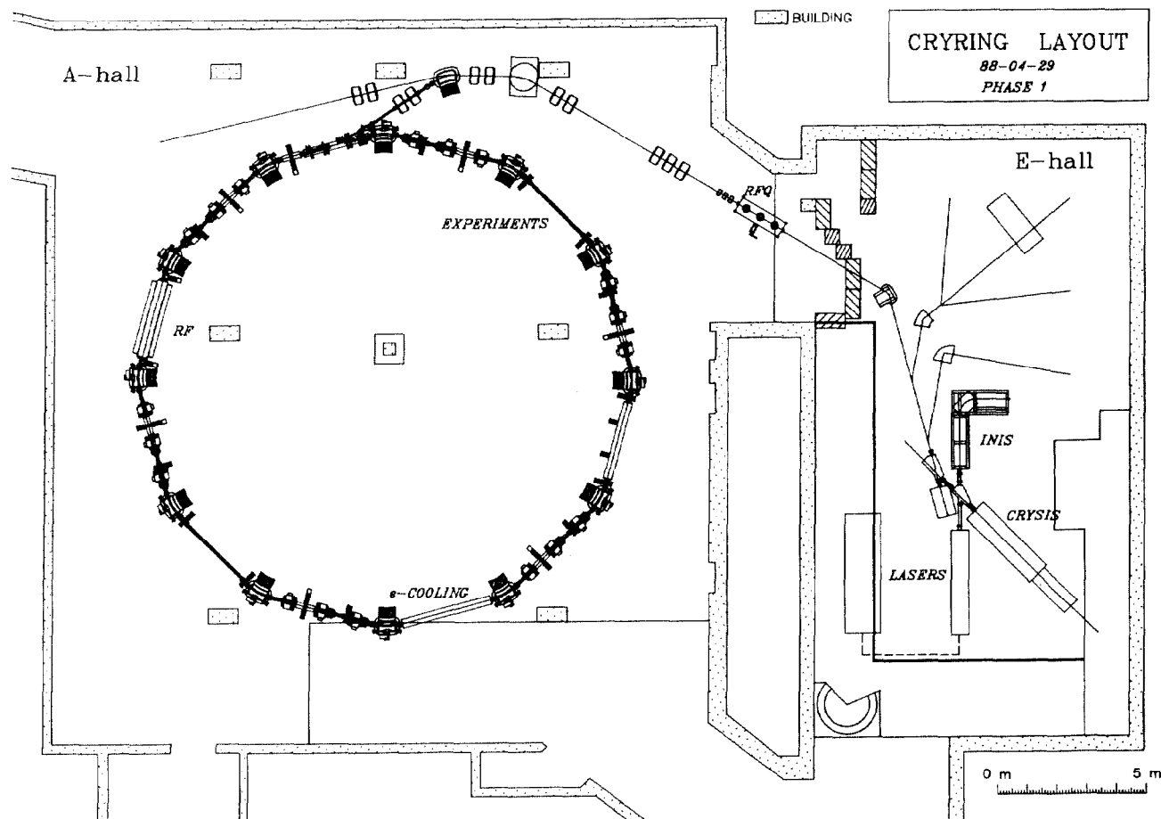
Fig. 1. Layout of the CRYRING facility.
