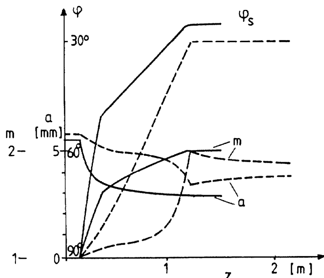
Fig. 3. The variation of the electrode parameters synchronous phase, \varphi_s , modulation, m and aperture, a along the z -axis. The dashed lines correspond to the old method of RFQ-design and the solid lines to the new method used in our design.
