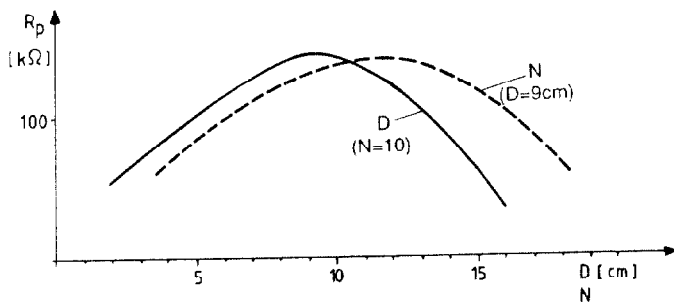
Fig. 5. Calculated R_p -value vs. stem diameter, D and number of stems, N .
