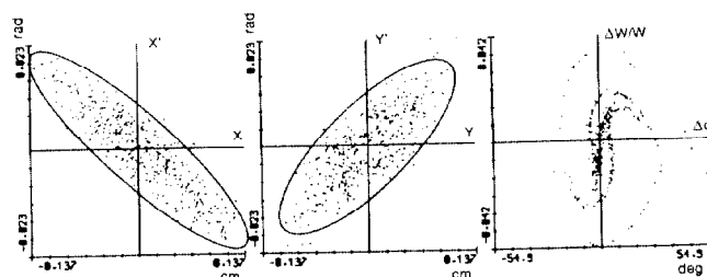
Fig. 4. Calculated phase space plots for the beam after the RFQ.
