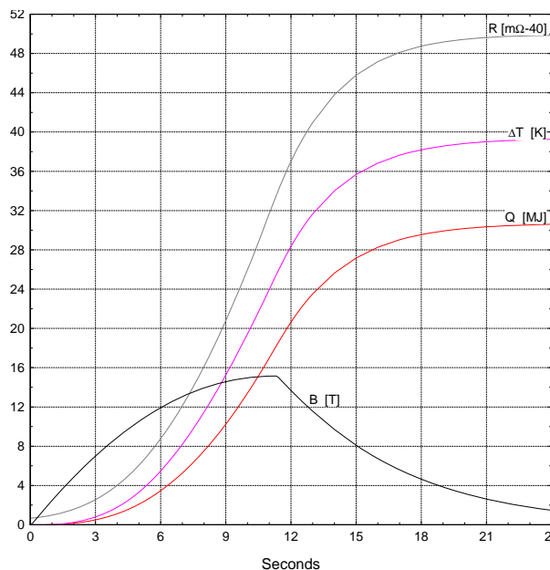
Figure 2: Calculated behavior of the 15-T magnet during a pulse. The peak current is 7200 A at a peak voltage of 700 V. Approximately 30 MJ of energy is dissipated in the magnet, which raises its temperature from 80 to 120 K.
