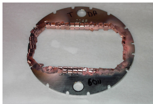
Figure 2: Rf seal damaged by beam-induced heating.
