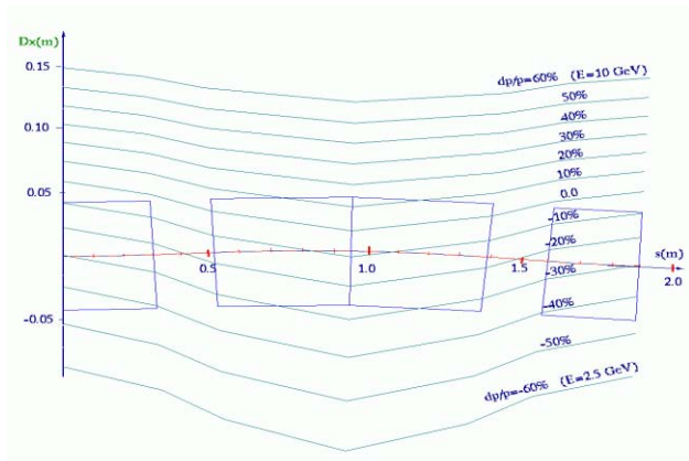
Figure 4: Dispersion function variation with energy.
