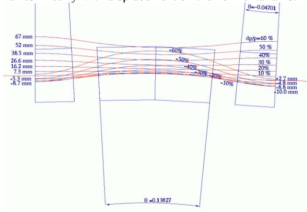
Figure 2: Orbit offsets during acceleration. The cell length is L_0=1.9 m.
