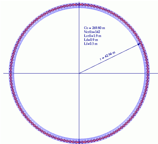
Figure 1: The NS-FFAG ring used for racetrack RLA return arcs, using 142 densely populated FODO cells of combined function magnets. The magnet lengths are L_D=0.9 \text{ m} and L_D=0.3 \text{ m} , with a drift of l_3=0.2 \text{ m} .
