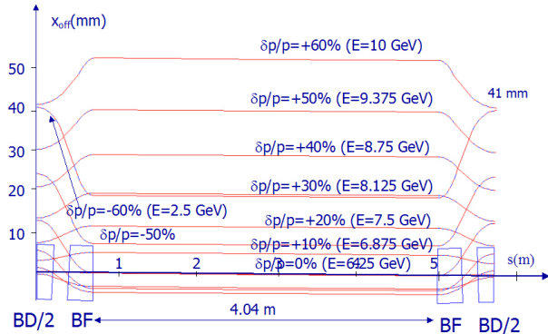
Figure 7: Large matching cell with orbits.
