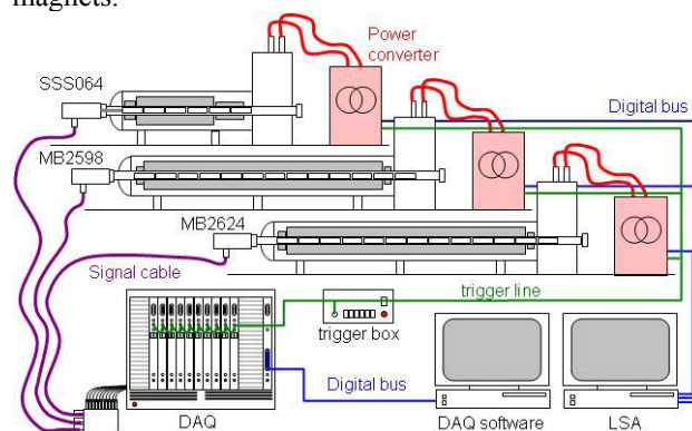
Figure 1: Set-up used for the measurement of the main field strength using the fixed coils.
