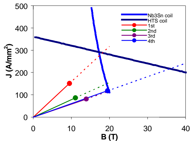
Figure 4: Critical coil current density and load lines for the 1 st , 2 nd , 3 rd and 4 th sections.
