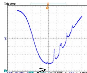
Figure 4: Cs transition from 6S_{1/2} to 6P_{3/2} Doppler free spectroscopy. the horizontal axis is proportional to the laser frequency while the vertical one shows the transmission through the Cs cell.
