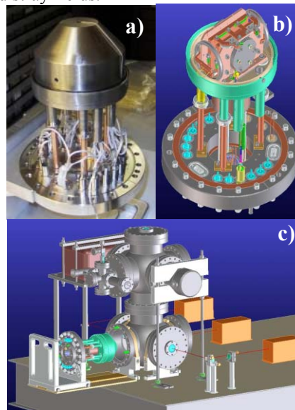
Figure 2: 3D CAD views and picture of DEGAS. a) The source fully assembled on the main flange (8" conflat) with the magnetic shield on. b) A view without the magnetic shield. c) The main flange with the source being inserted into the main vacuum chamber. The 3 laser boxes in orange are also visible.
