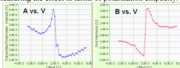
Figure 5: Signal at the polarimeter exit (point A in Fig. 3) and its first harmonic (point B in Fig. 3). Quarter wave plate in.
