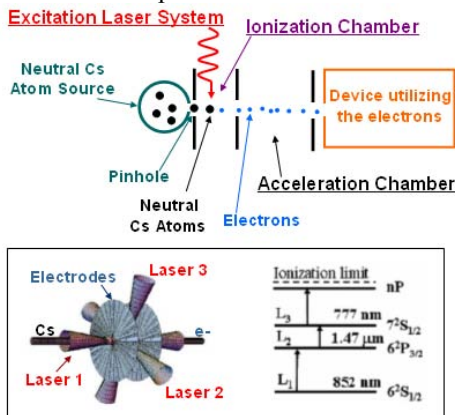
Figure 1: Source layout and Cs atom excitation scheme.
