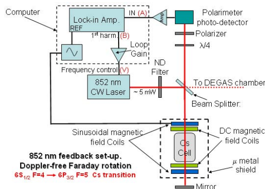
Figure 3: Frequency feedback scheme for the 852 nm laser.
