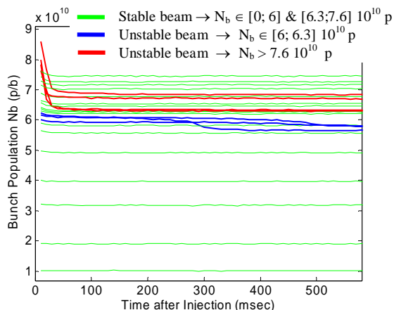
Figure 2: Bunch intensity vs. time for a bunch with low longitudinal emittance ( \varepsilon_L = 0.16 \text{ eVs} ).
