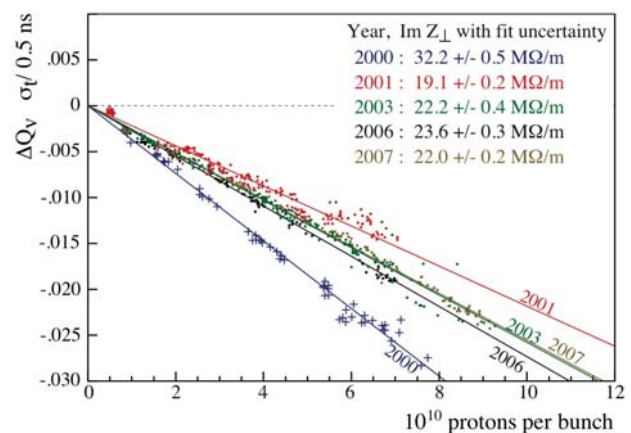
Figure 1: Measurements of the single-bunch vertical coherent tune shift vs. intensity over the last years.
