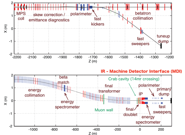
Figure 1: Layout of BDS functional subsystems[1].
