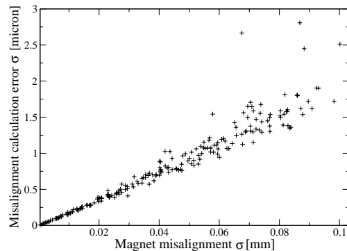
Figure 4: Dependence of standard deviation in magnet misalignment calculation on the standard deviation of the input magnet misalignments. Each data point uses a different misalignment error pattern. The BPM measurements are assumed to be perfect.
