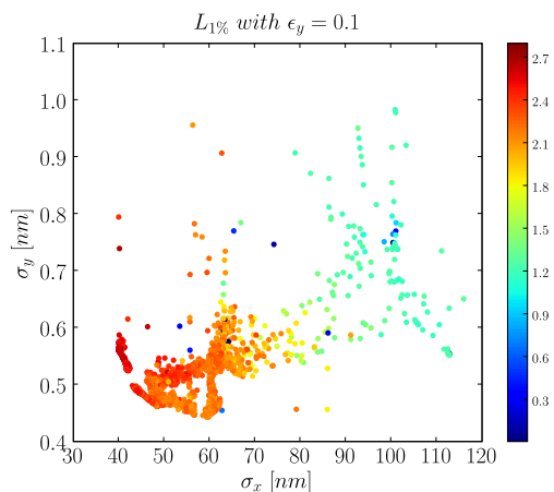
Figure 2: Peak luminosity per bunch crossing taking into account synchrotron radiation effects versus horizontal and vertical beam sizes. Peak luminosity is in arbitrary units and has an uncertainty of 5%.
