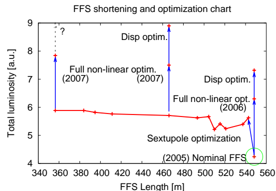
Figure 1: Chart of the optimization of the CLIC Final Focus System showing total luminosity versus the length of the FFS. The starting point is the nominal configuration in 2005. Optimizations are: sextupole, full non-linear, dispersion. Optimizations on top of length reductions prove successful. Dispersion optimization was not computed for the shortest system.
