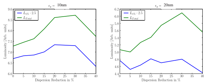
Figure 4: Plots for \sigma_z = 44\mu\text{m} , showing the total and peak luminosities versus dispersion reduction. The left plot has a vertical emittance of 0.01\mu\text{m} while the right plot has 0.02\mu\text{m} .
