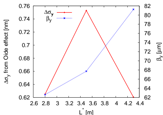
Figure 7: Increase in the IP vertical beam size caused by considering synchrotron radiation in the final doublet versus L^* . All cases have \epsilon_{y0} = 20\text{nm} .
