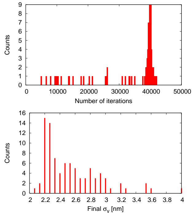
Figure 6: Histograms of vertical beam sizes (before and after correction) and iterations taken by the optimization for the CLIC FFS. Figure of merit: Beam size plus non-linear dispersion. knobs: H&V displacements plus strengths
