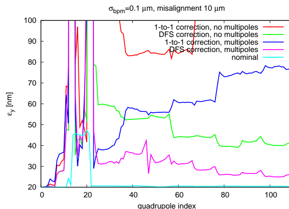
Figure 2: Vertical emittance versus longitudinal location after attempting the alignment of the full CLIC BDS by one-to-one steering and dispersion free steering.
