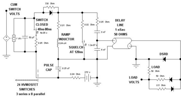
Figure 2: Schematic design of kicker driver, DSRD and load at right.
