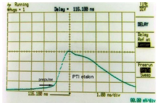
Figure 4: Reverse voltage pulse of Ioffe Physics Institute's PTI etalon DSRD diode. Forward pumping is 100 nanoseconds in duration. Avalanche occurs at 500V. Time-axis: one nanosecond per division.
