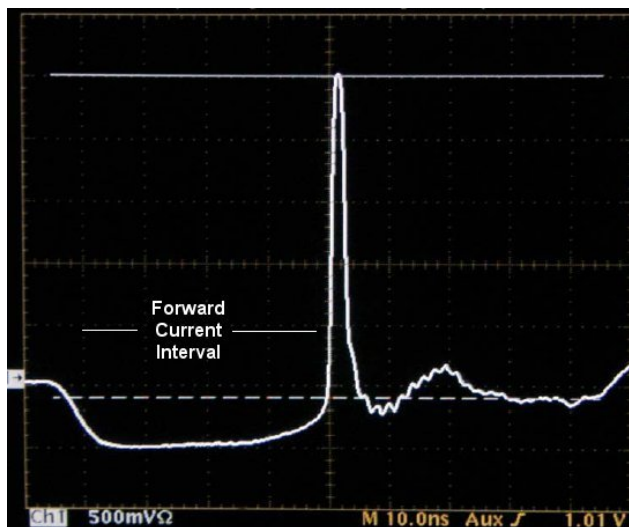
Figure 5: Pump and step recovery switching performance of DSRD stack provided by Ioffe Institute of Physics, compliments of Professor Alexei Kardo-Sysoev. Time axis 10ns/division. Peak voltage 1000V; one-nanosecond delay line employed.
