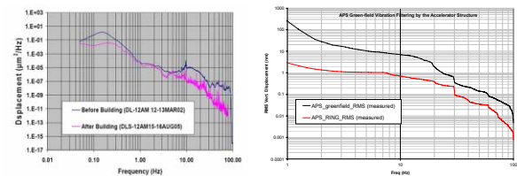
Figure 15: Observed filtering of motion (DLS and APS)
