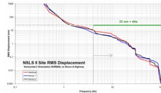
Figure 8: Site rms displacement and ring criteria .
