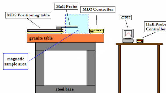
Figure 2: Diagram of the mapper's main parts.
