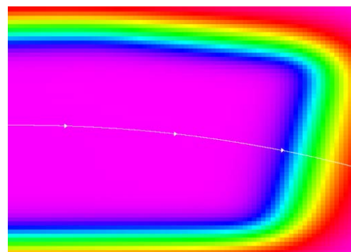
Figure 5: The orbit of an electron in the B-field of a bending magnet.
