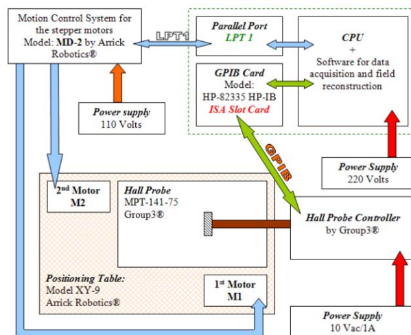
Figure 1: The mapping device block diagram.
