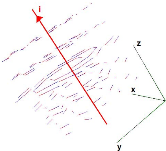
Figure 6: Linear current's reconstructed field.
