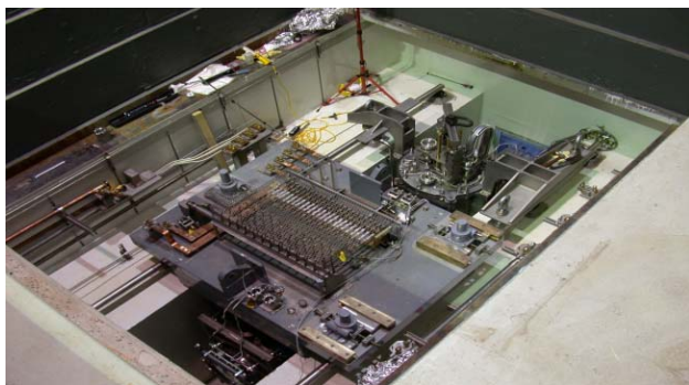
Figure 3: Rad-Hard Quadrupole & Diagnostic Installed.
