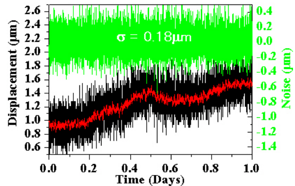
Figure 4: The signal observed in the EM noisy place; cable length is 50m and HLS made by FOGALE. in the high EM noisy place and the root mean square [rms] noise width becomes 0.18\mu\text{m} .
