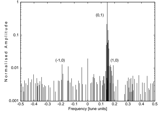
Figure 4: Vertical Fourier spectrum for compensation.
