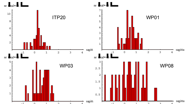
Fig. 4: The sagitta of magnets having been measured at all four work-packages, ITP20, WP01, WP03 and WP08
