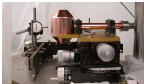
Figure 2: Fiducialization of a drift tube.
