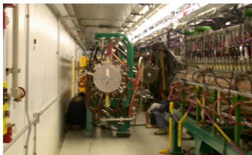
Figure 1: DTL 4 moving into place.
