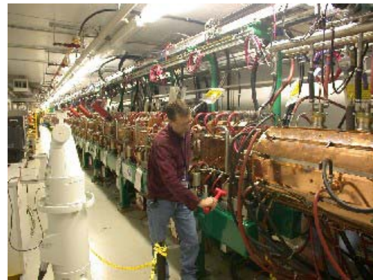
Figure 8: CCL magnet alignment.
