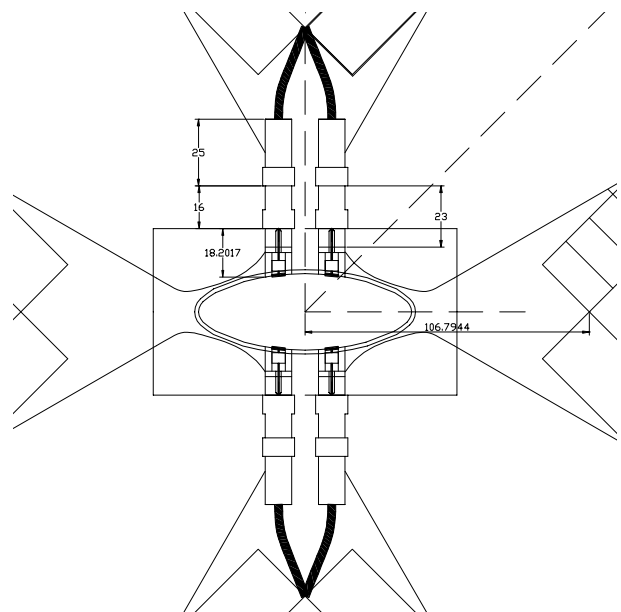
Figure 4. Layout of pick-up monitor installation in NESTOR.
