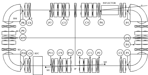
Figure 2. Layout of pick-up and corrector location along NESTOR orbit: P1-12 – pick-up monitors; C1-C9 – correctors in sextupole magnets.
