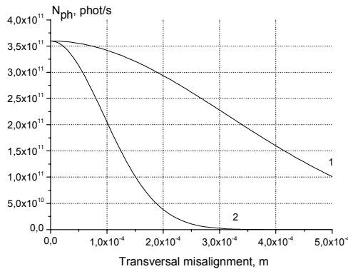
Figure 5. Scattered radiation intensity vs transversal mismatching of electron and laser beam position. 1 - mismatching in horizontal plane; 2 - mismatching in vertical plane.
