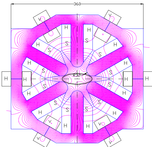
Figure 3. Layout of sextupole magnet with corrector coils.
