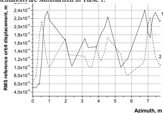
Figure 1. RMS value of reference orbit displacement along NESTOR orbit on a half of circumference.
