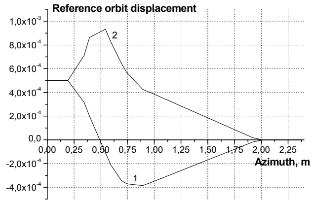
Figure 6. Reference orbit displacement for compensation of lattice element alignment effect vs NESTOR azimuth from the IP till the first bending magnet enter: 1 - in horizontal plane, 2 - in vertical plane.
