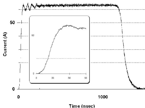
Figure 5: A 10%-90% risetime of 26 ns is achieved with a 6.2 kV pulse into a 100 \Omega load with the grid pulser circuit.
