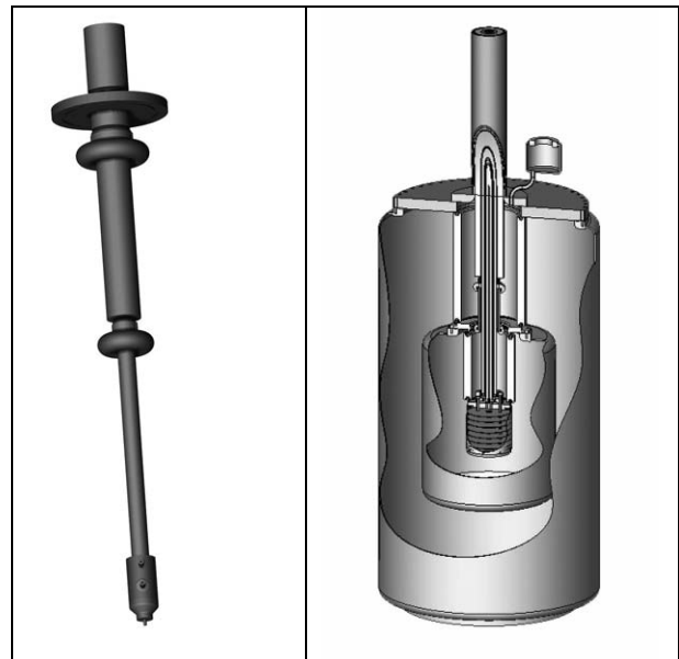
Figure 3: (left) Conventional corona shield and tapered dielectric expansion construction is used to terminate the cable at the HV source tank. (right) A novel re-entrant socket is built into the klystron gun, making an inverted direct compact interconnect between cable and klystron.
