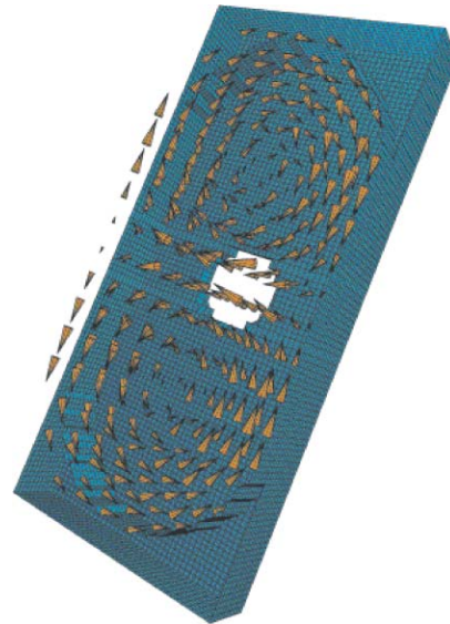
Figure 2: Magnetic field distribution of the lowest dipole mode of transverse deflection in a racetrack shape cavity. (Beam deflecting mode).
