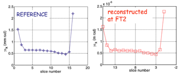
Figure 5: Reconstructed horizontal beam slice emittance (in mm-mrad) as a function of slice number with the beam size scanning at FT2. The left curve is the horizontal emittance as calculated by slicing the beam output file (tracked with Elegant) along the temporal coordinate, the right curve is the result of the simulated quadrupole scan at the screen location.
