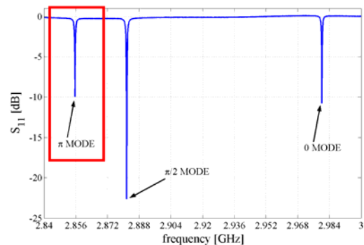
Figure 9: Measured reflection coefficient at the input coupler port.
