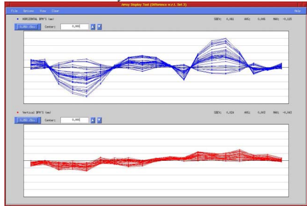
Figure 4: Horizontal (top) and vertical orbit modulation with a single shunt AC excited.
