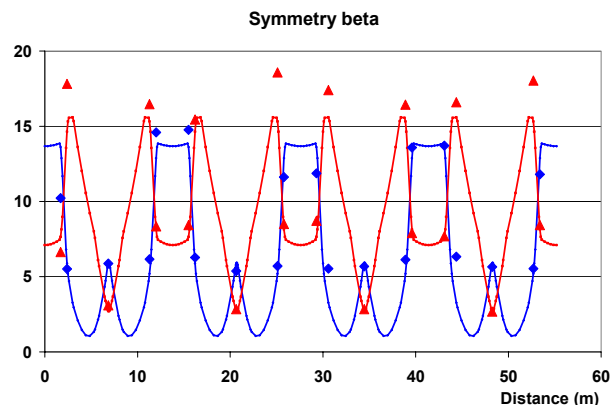
Figure 6: Measured beta values (points) compared with the model lattice (solid lines).
