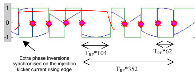
Figure 4: example of a cleaning signal (blue) with no DC component over 2 revolutions, for v_H=0.2 and four bunches accelerated (red: injection kick signal, pink: bunches)
