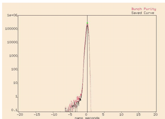
Figure 6: bunch purity measured on a beam stored in the SR after cleaning in the booster
