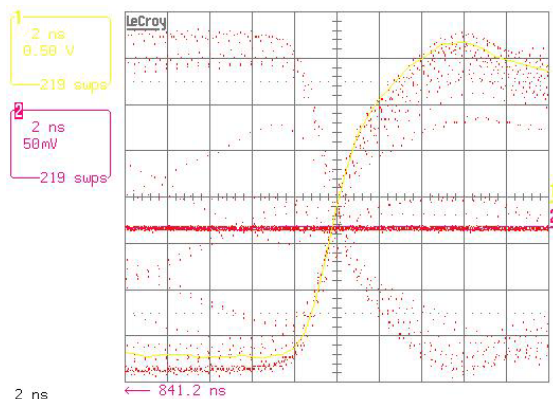
Figure 5: high power stripline signal rise and fall time during the phase inversions (2ns/div).
