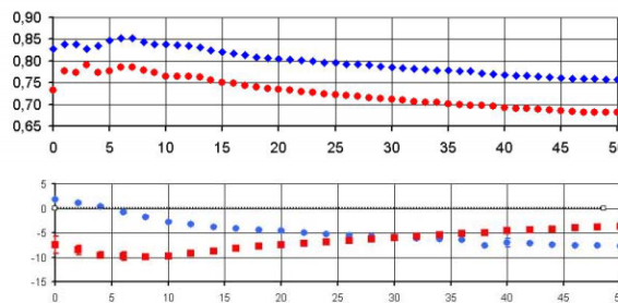
Figure 2: SY booster horizontal (blue) and vertical (red) tune (upper) and chromaticity (lower) during the 50 ms acceleration cycle.
