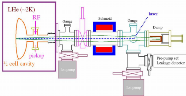
Figure 5. Test setup for quantum efficiency measurements of all niobium SC RF gun.
