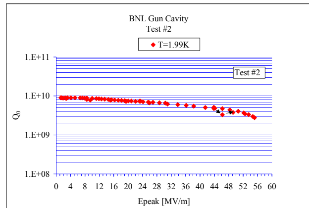
Figure 4. Results of cavity field measurements after chemical polishing and high pressure rinse.
