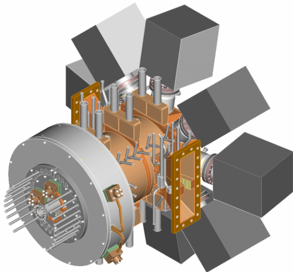
Figure 2. Engineering model of the normal-conducting CW RF gun.
