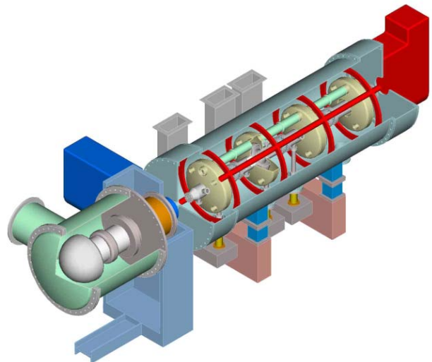
Figure 1. Engineering model of the DC gun and SRF cryomodule high-power CW injector.
