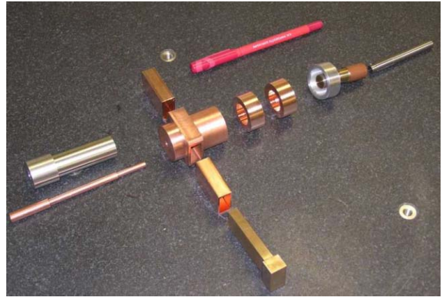
Figure 6. X-band gun cold model parts prior to assembly.
