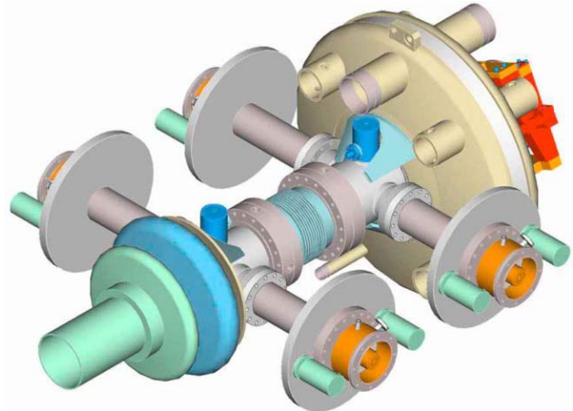
Figure 3. Half cell SRF gun followed by a booster accelerating cavity.
