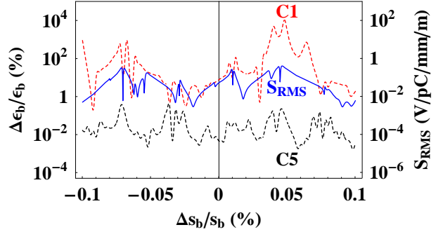
Figure 3: Emittance dilution, \Delta \epsilon_b / \epsilon_b , for a single class of cavities (C1 shown in red) and for five classes of cavities (C5 shown in black). The RMS of the sum wakefield, S_{RMS} , is also illustrated for a single class of cavities (shown in blue).
