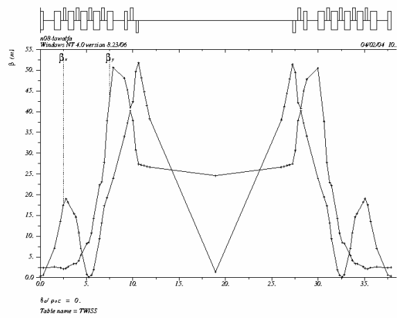
Figure 3a: beta-functions at 490 MeV
