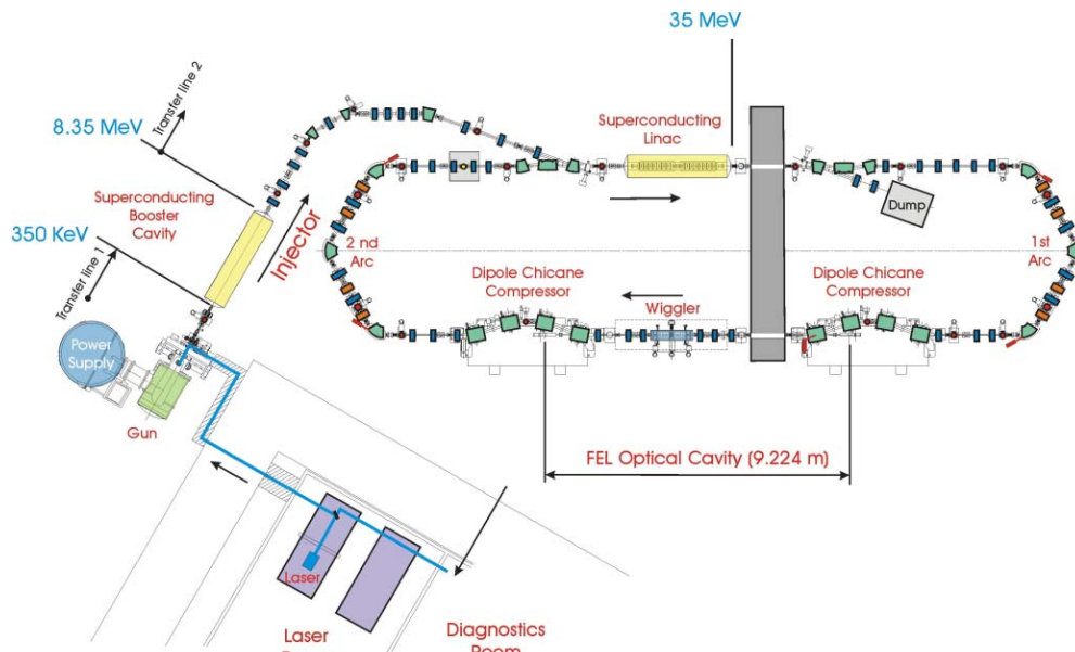
Figure 1: Layout of Daresbury Energy Recover Linac Prototype.
