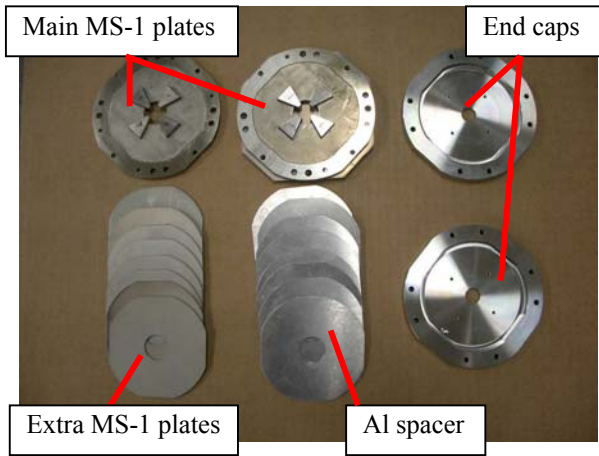
Figure 4: Temperature compensation parts
