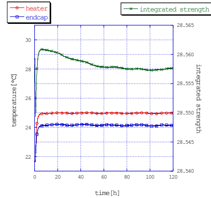
Figure 6: Measurement of the PMQ with 4 extra MS-1 plates
