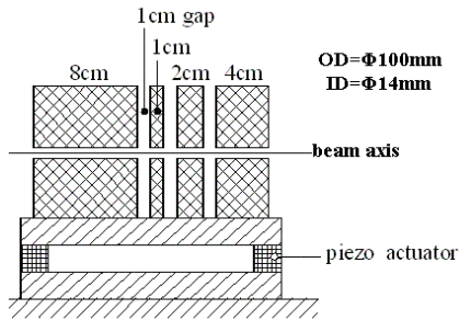
Figure 8: Strength Adjustable PMQ.
