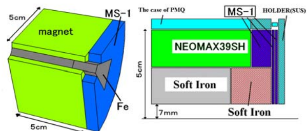
Figure 3: PMQ with compensation add-on part
