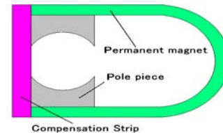
Figure 2: An example of temperature compensation with compensation material. Compensation strip shunts the flux.
