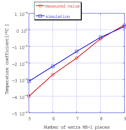
Figure 7: Measured and calculated values of temperature coefficient with various numbers of MS-1 plates
