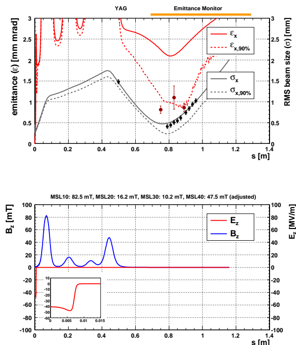
Figure 3: Top: Comparison of simulation results (solid and dashed lines) with measurements (points with error bars). See text for details. Bottom: Magnetic and electric field strengths entering the simulation drawn on the same horizontal scale.
