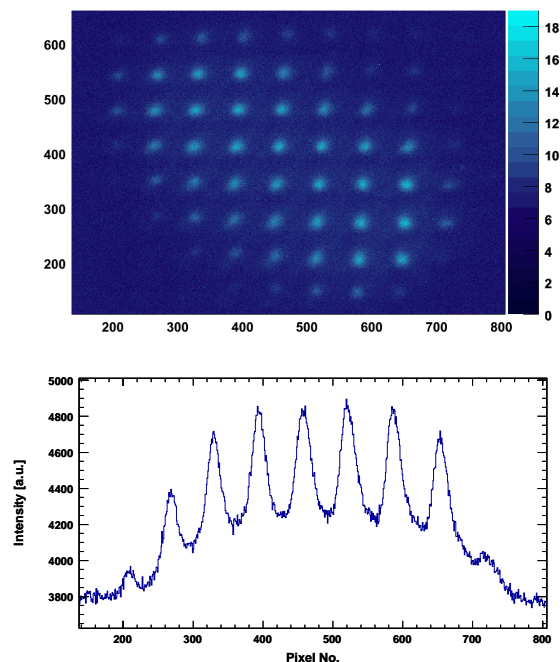
Figure 2: Detail of a typical pepper-pot raw image (top) with corresponding projection (bottom).
