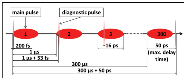
Figure 3: Time scheme of the scanning cross-correlator used for 3-D laser pulse diagnostics.
