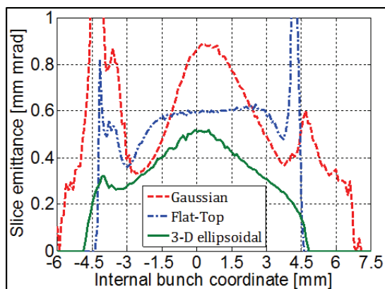
Figure 1: Beam dynamics simulation of electron bunches for photo cathode laser pulses with flat-top, Gaussian and 3-D ellipsoidal temporal profiles; left: normalized transverse slice emittance \epsilon_{slice} distribution along the electron bunch, right: values of normalized transverse projected emittance \epsilon_{proj} and normalized average slice emittance \langle \epsilon_{slice} \rangle .
