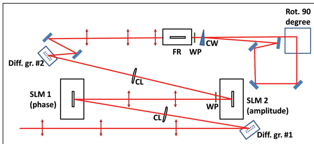
Figure 2: Setup of the 3-D pulse shaper: Diff. gr. – diffraction gratings, SLM – spatial light modulator, WP – half-wave plates, CL – cylindrical lens, FR – Faraday rotator, CW – calcite wedge, Rot. 90 degree – laser beam rotator (90°).
