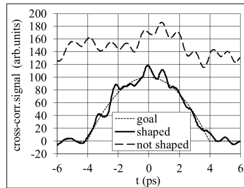
Figure 4: Scanning cross-correlator measurements of pulses w/o pulse shaping (dashed line), w/- amplitude mask pulse shaping (solid line) and aspired profile (dotted line).
