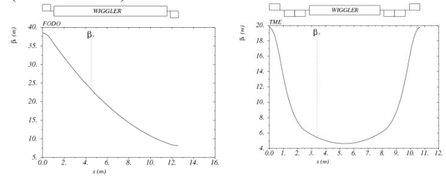
Figure 2: Two wiggler cells: FODO (left) and TME-like.
