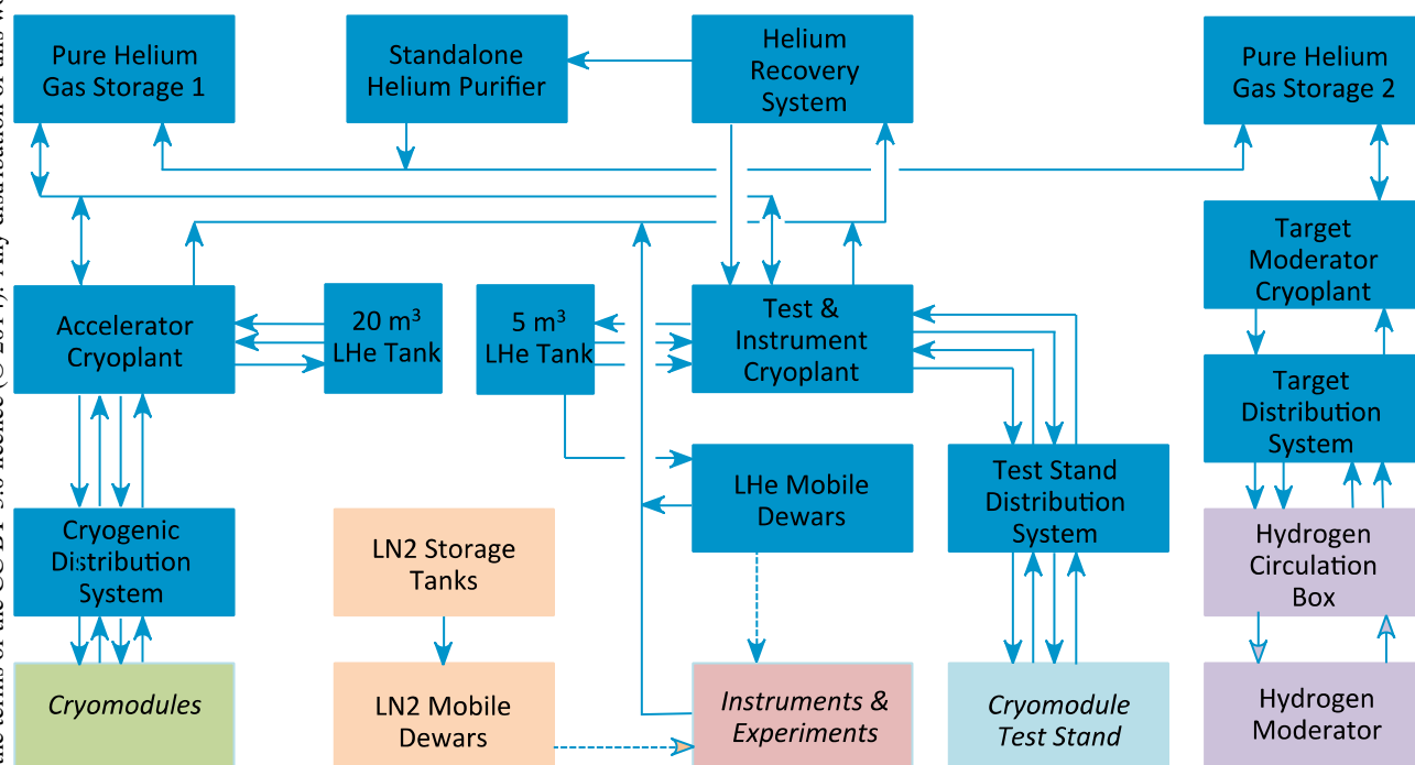
Figure 1: ESS Cryogenic System Block Diagram.
