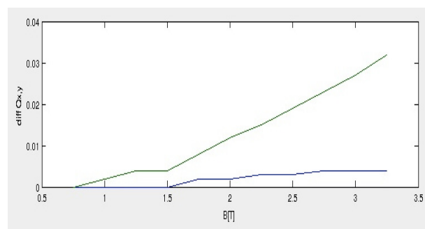
Figure 5: Horizontal (blue) and Vertical (green) Tune Shift.
