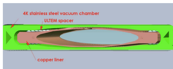
Figure 3: Cross section of the wiggler vacuum chamber and the copper liner.
