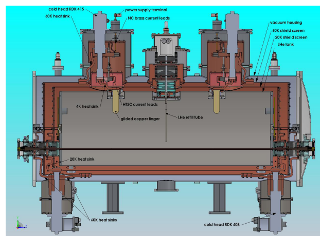
Figure 2: Superconducting wiggler cross section.
