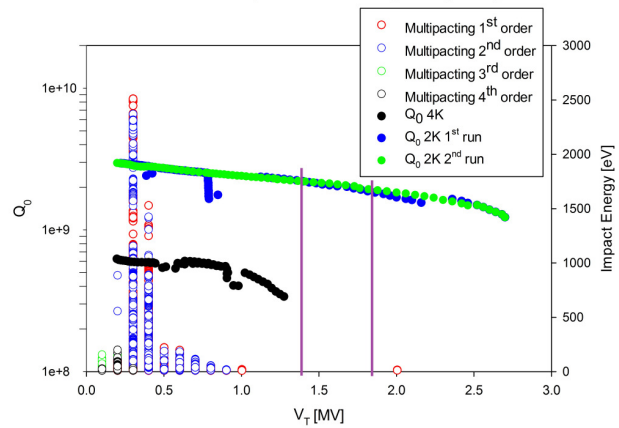
Figure 3: Q_0 measured at 4 K (solid black) and 2 K (solid blue and green) compared to the multipacting levels obtained from the TRACK3P-ACE3P simulations. The purple lines enclose the crabbing kick range needed per cavity in the MEIC.
