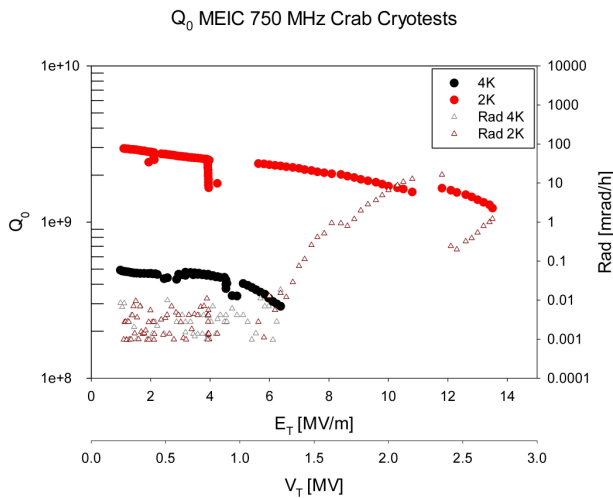
Figure 2: Measured quality factor showing the multipacting barriers and radiation generated during the 4 K and 2 K cryogenic tests. An event around 12 MV/m shows the burst of a field emitter that produces an abrupt reduction (2 orders of magnitude) in the X ray production.
