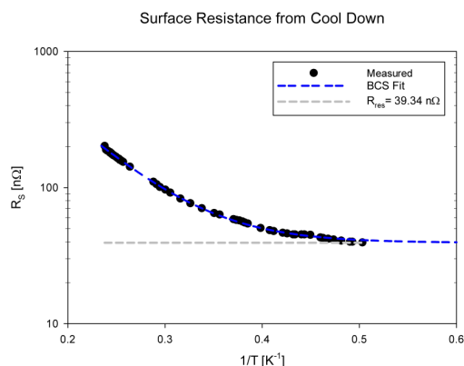
Figure 6: Residual surface resistance calculated using the effective surface resistance data measured during the cavity cool down and fitted to the BCS theory.
