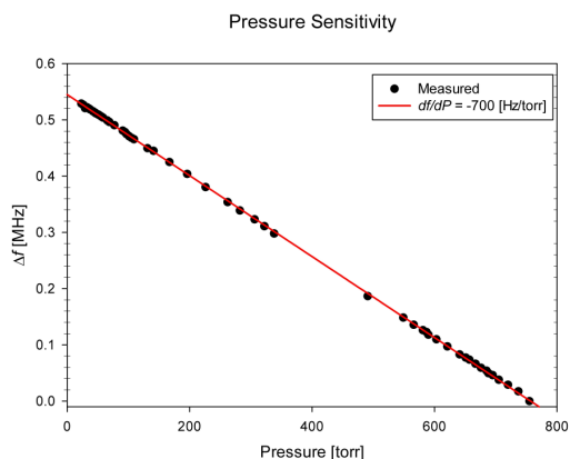
Figure 5: Pressure sensitivity from measurements of the resonant frequency shift during the liquid Helium pump down in the Dewar (from 760 to 23 torr).
