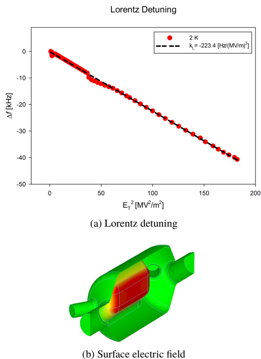
Figure 4: Lorentz coefficient from measurements of the resonant frequency shift during cool down (a). Cross section showing the electric surface fields from simulations, placed on the flat area of the loading elements (b).
